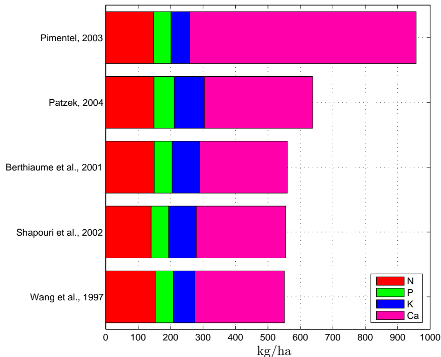
Figure 4: The total fertilizer application rates listed in Tables 3, 5, 7, and 8.
