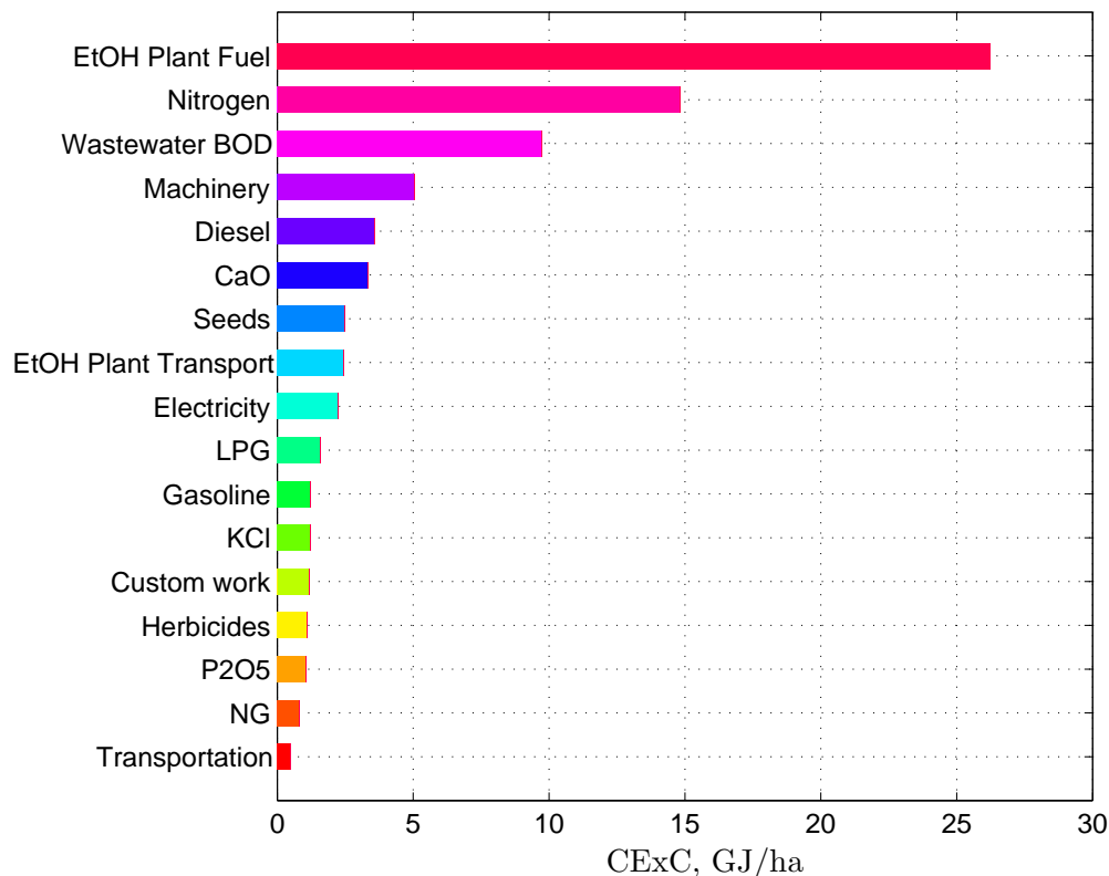
Figure 41: The specific cumulative exergy consumption (CExC) by each major non-renewable resource input to the industrial corn-ethanol cycle.
