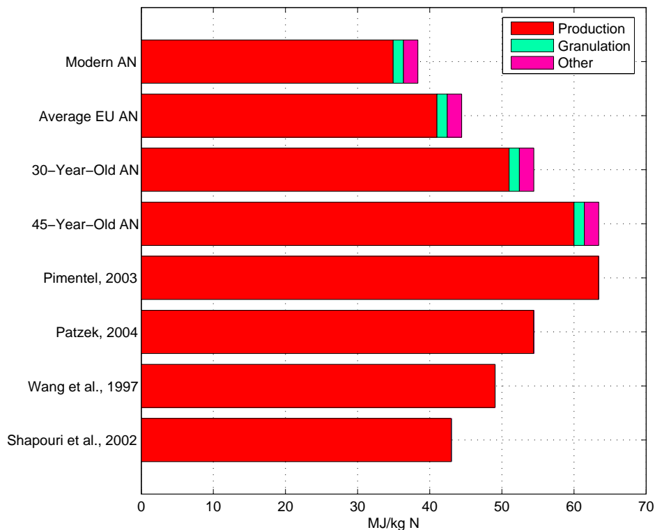
Figure 3: The various estimates of the unit energy consumption to produce ammonium nitrate (AN). The estimates by SHAPOURI et al. are listed in (Shapouri et al., 2002), by WANG et al. in (Wang et al., 1997), and PIMENTEL's estimate (Pimentel, 2003) of 78.1 MJ/kg N was adjusted down to the 45-year-old AN.
