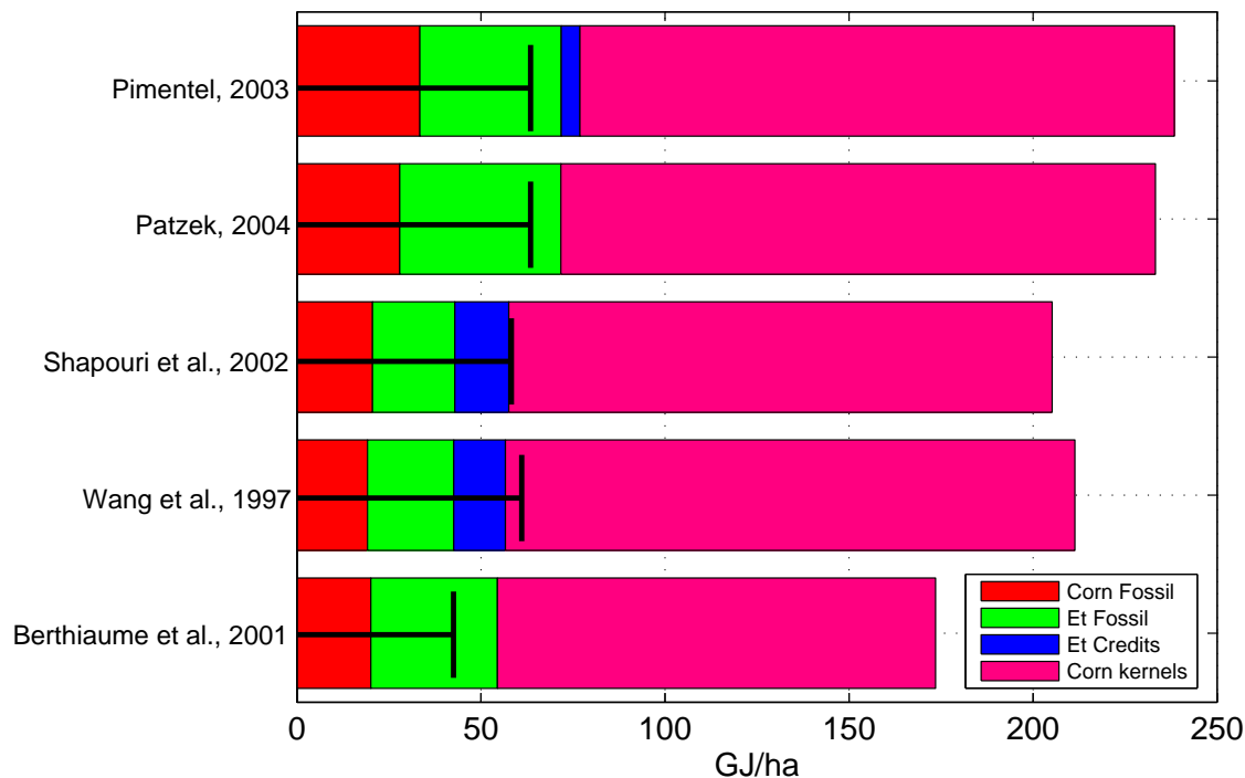
Figure 16: The overall energy balance of ethanol production. The two or three leftmost parts of each bar represent the specific fossil energy used in corn farming and ethanol production. The fossil energy inputs into ethanol production are the sum of the green part and the blue energy credit part for some authors. The rightmost part is the calorific value of corn grain harvested from 1 hectare. The total lengths of the horizontal bars represent all energy inputs into ethanol production. The horizontal lines with the vertical anchors represent the calorific value of ethanol obtained from one hectare of corn. Note that the total energy inputs into ethanol production are equivalent to over 4 metric tonnes of gasoline per hectare. The ethanol's calorific value is equal to 1 metric tonne of gasoline.
