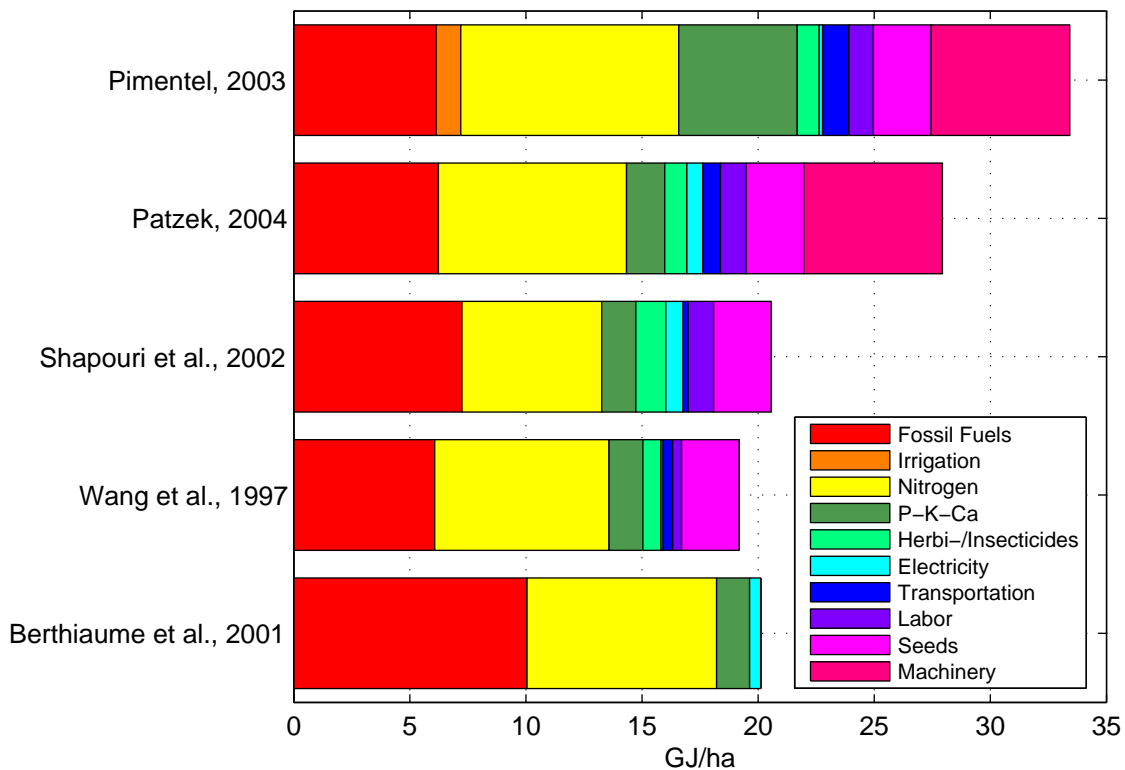
Figure 11: Major fossil energy inputs into corn farming.
