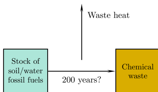
Figure 26: Current industrial agriculture is another example of a linear process, which by definition cannot be sustainable.
