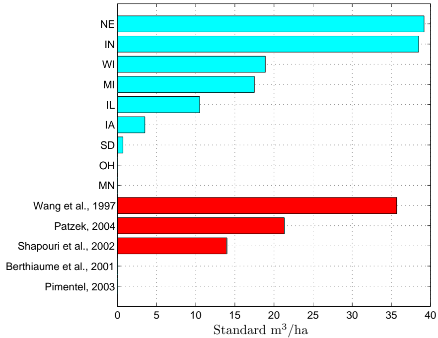
Figure 7: By-state and average use of methane in corn farming. The 1996 methane volume data from the largest corn-producing states are from SHAPOURI et al. (2002). Note the large variability of methane use depending on wet/dry weather.
