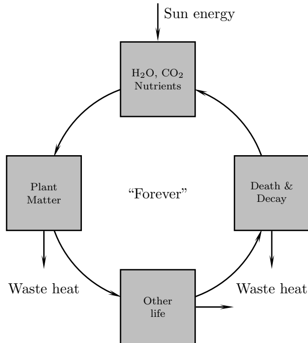
Figure 27: An ecosystem transforms the sun energy (low thermal entropy) into waste heat (high thermal entropy). The waste heat is continuously exported to the universe. Everything else is completely reused, or recycled.
