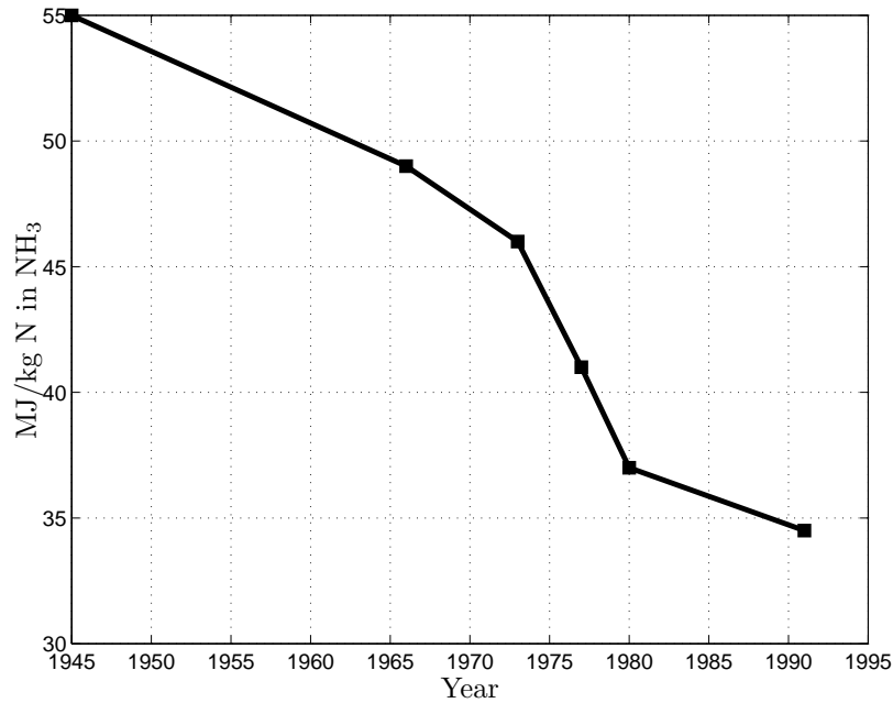
Figure 1: History of energy efficiency of ammonia production in MJ/kg N. Source: G. KONGSHAUG (1998).
