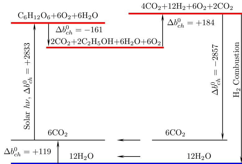
Figure 39: Exergy diagram of the ideal CO 2 -Glucose-EtOH-H 2 cycle.
