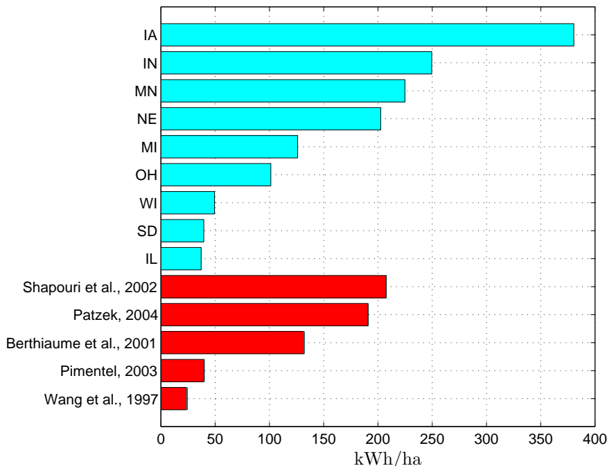
Figure 8: By-state and average use of electricity in corn farming. The 1996 electricity data from the largest corn-producing states are from SHAPOURI et al. (2002). Note the large variability of electricity use depending on wet/dry weather.
