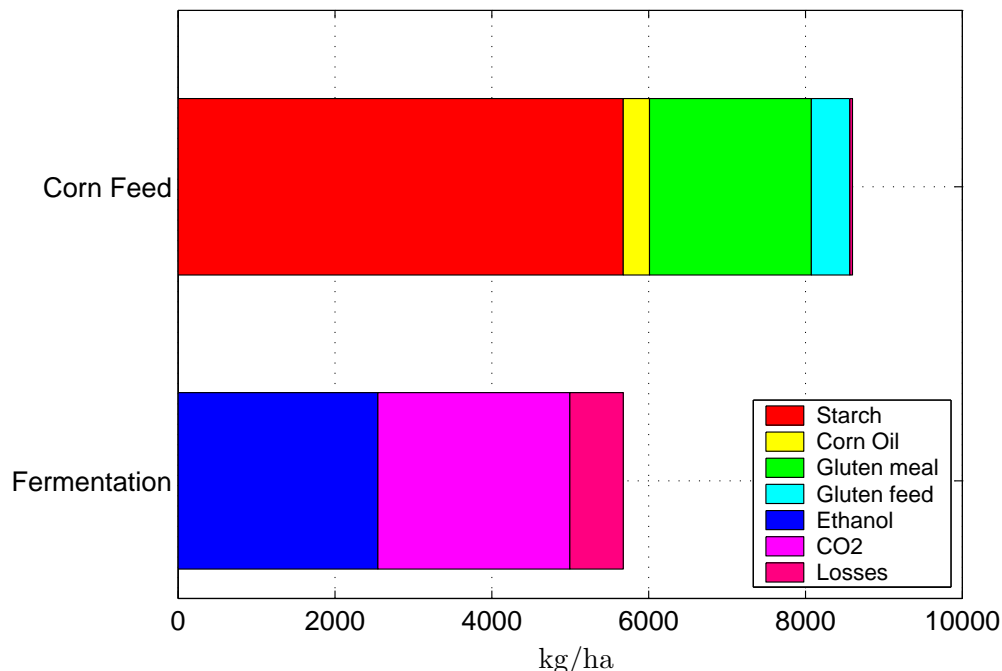
Figure 13: The result of practical corn conversion into ethanol is 0.372 L EtOH/kg dry corn grain = 2.50 gal EtOH/ dry bushel = 2.18 gal EtOH/ wet bushel with 15% moisture.
