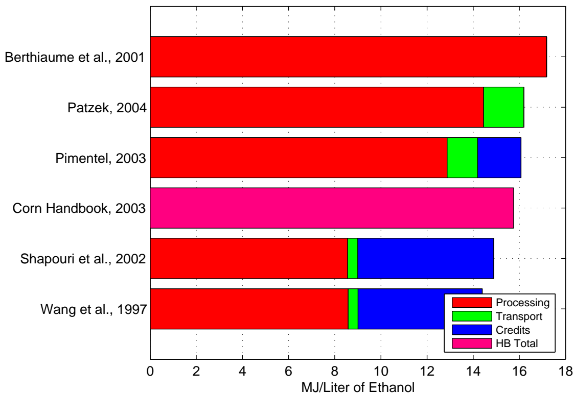
Figure 15: The average fossil energy inputs to ethanol production in a wet milling plant. The length of each bar is the total energy outlay to produce 1 liter of EtOH, and the blue parts denote the size of energy credits assumed by the different authors.
