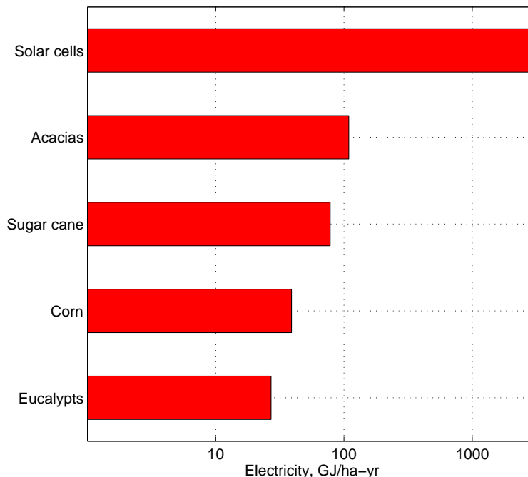
Figure 45: The amount of electricity generated in 1 year with solar cells on 1 ha dwarfs those generated with hydrogen-burning 60%-efficient fuel cells or in power stations. The hydrogen is obtained with no losses from ethanol from corn and sugarcane, and electricity is generated with the 35%-efficiency from eucalypt and acacia wood pellets. The annual electricity yields have been calculated by PATZEK & PIMENTEL (2005). The minimum solar cell yield follows the assumptions in this appendix. Note that the bar scale is logarithmic , and annually the solar cells produce \sim 100 times more electricity than corn ethanol.
